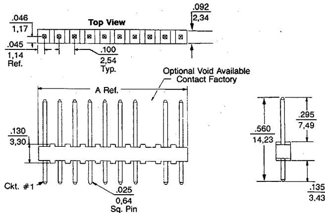
Recommended P.C. Board Layout for .100" (2.54 mm) Headers
