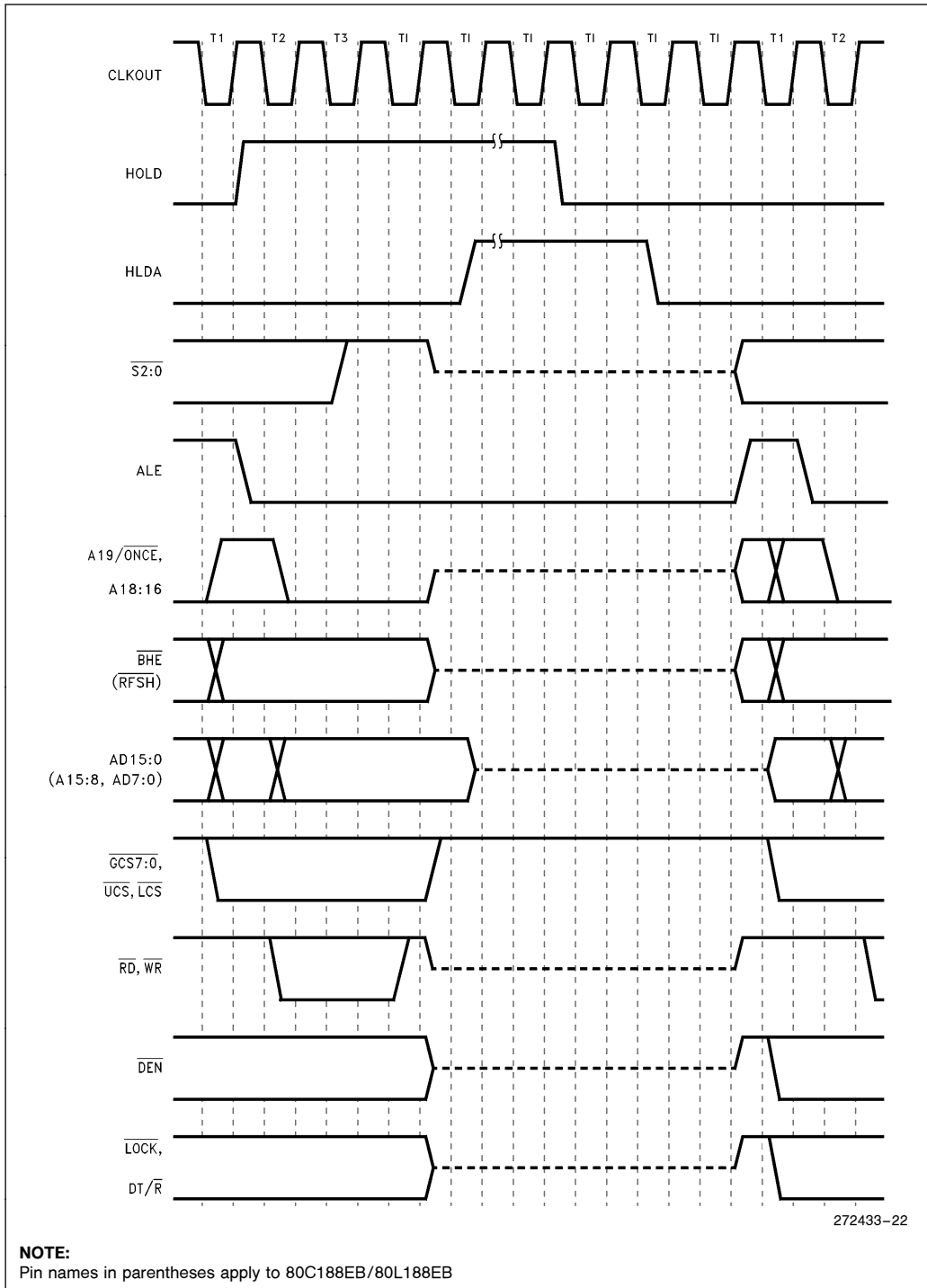
Figure 21. HOLD/HLDA Waveforms
