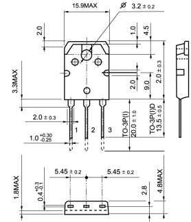
TO-3P(I)D
